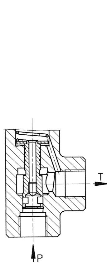
Fig. 1: Sectional drawing
